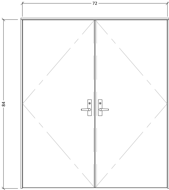
2 ELEVATION 1/2" = 1'-0"
