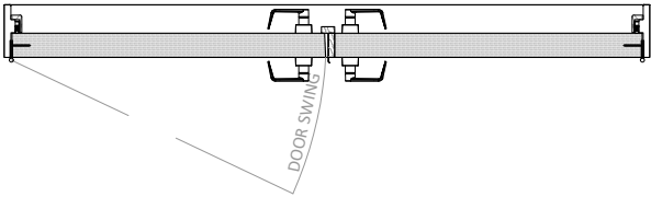
3 PLAN 1/2" = 1'-0"
