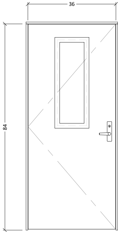
2 ELEVATION 1/2" = 1'-0"
