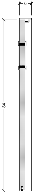
1 SECTION 1/2" = 1'-0"
