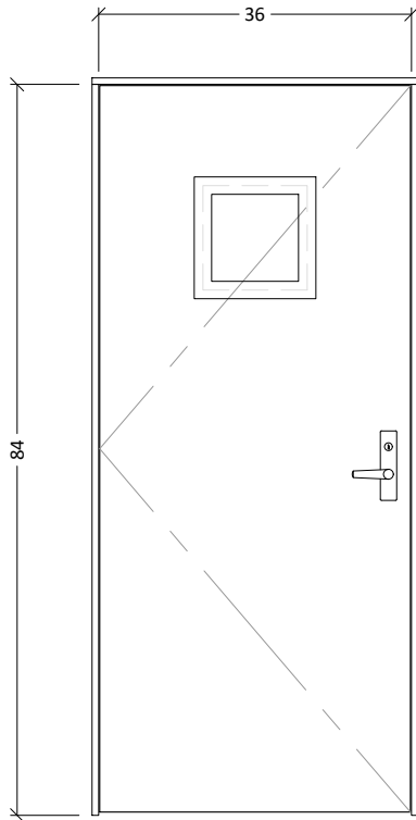
2 ELEVATION 1/2" = 1'-0"
