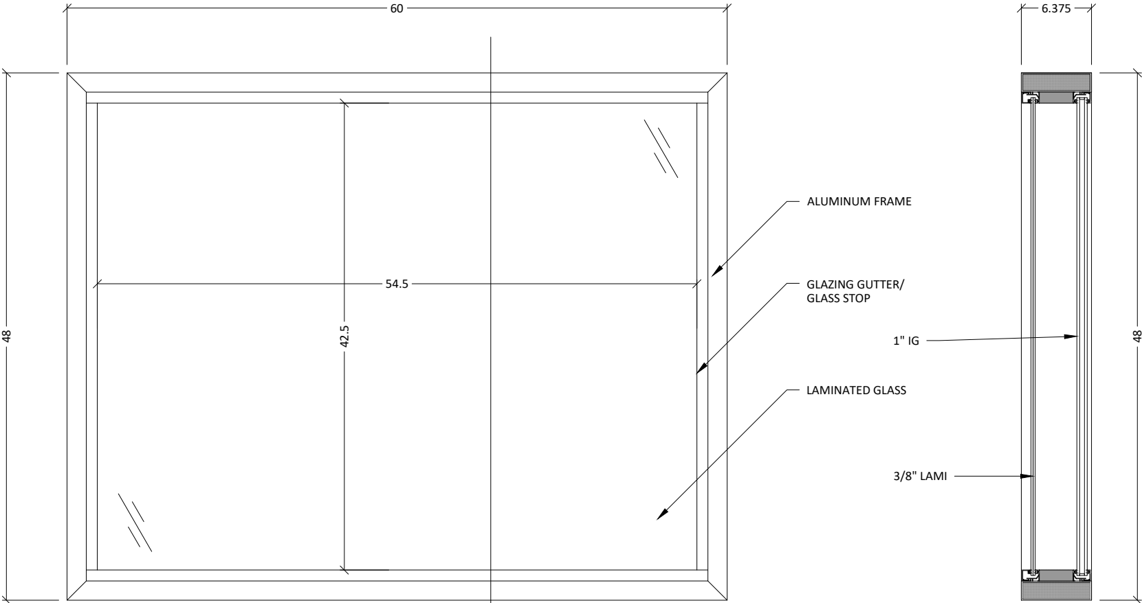
1 ELEVATION 1" = 1'-0"
