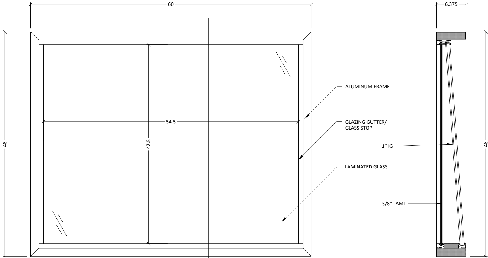
1 ELEVATION 1" = 1'-0"
