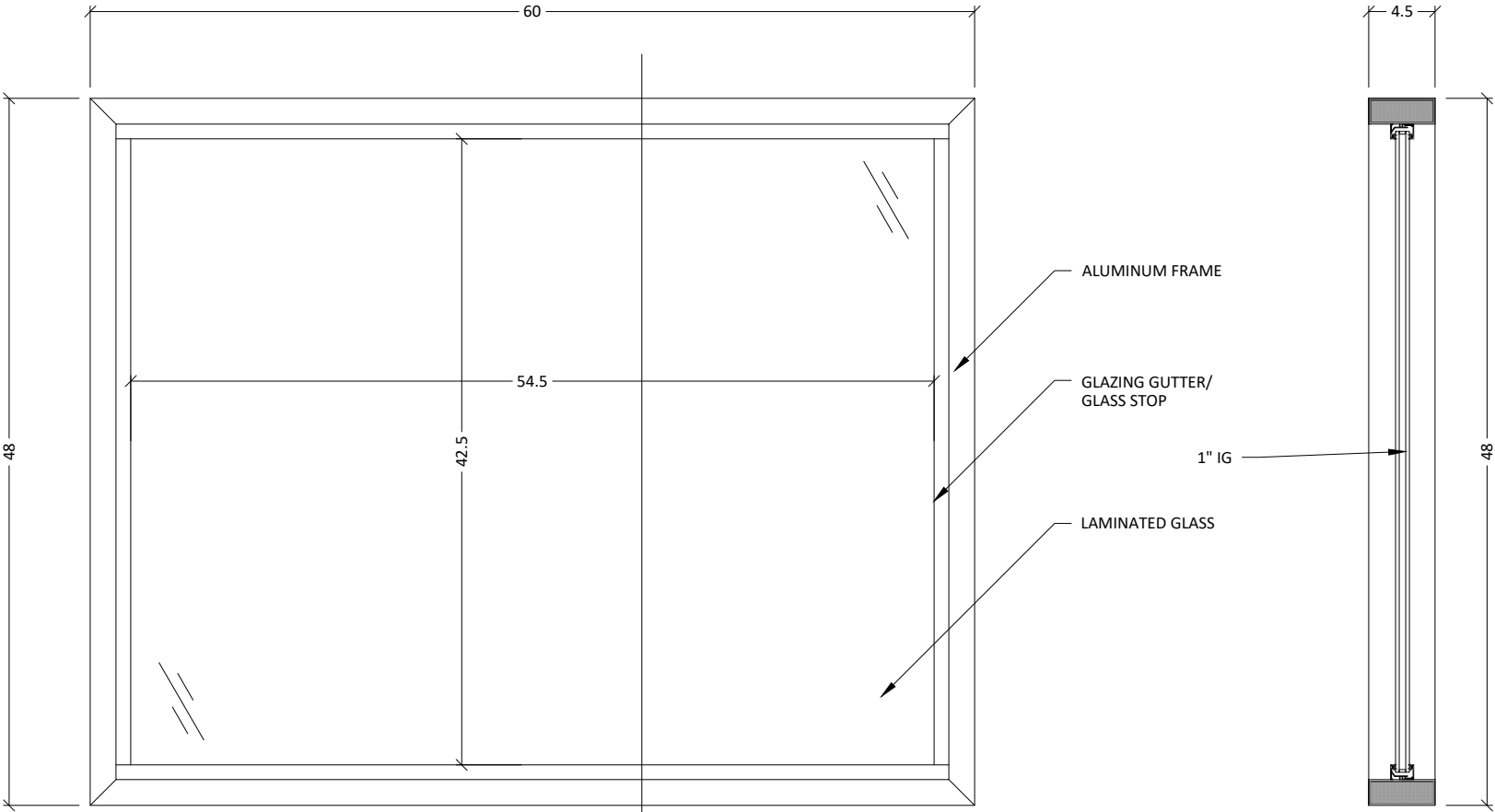
1 ELEVATION 1" = 1'-0"
